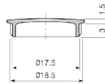
Cover Ø18 mm.
