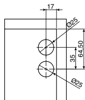
Rear drilling pattern for active safety version. Two possibilities.
