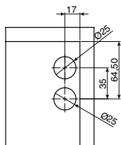
Rear drilling pattern for active safety version. Two possibilities.
