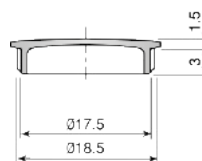
Cover Ø18 mm.
